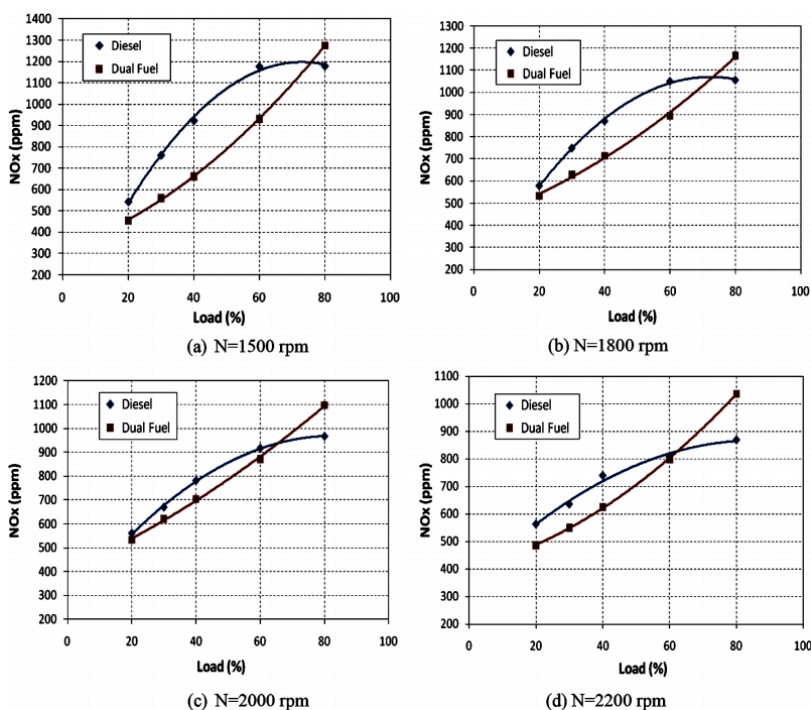
Figure 2. Variation of NO x emission according to load at different engine speeds (Lounici et al., 2014)
