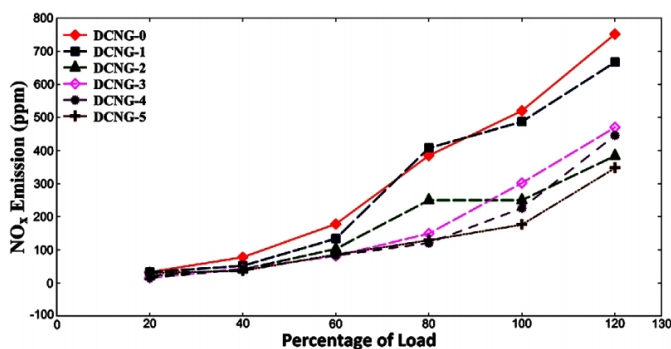
Figure 1. Variation of NO x emission with load for D-CNG combination (Paul et al., 2013)
